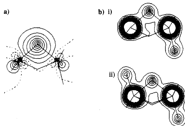
Figure 8. (a) Localized molecular orbital corresponding to the in-plane three-center, two-electron hydrogen bridging bond in the C_s(1) isomer. (b) Plot of total electron density in the C_s plane of the C_s(1) isomer (i) and plot of the total density in the plane of one of the remaining bridging hydrogens of the C_s(1) isomer (ii). Contour increments in (a) and (b) are 0.05 \text{ bohr}^{3/2} and \text{bohr}^3 , respectively.
