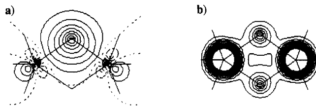
Figure 7. (a) Localized molecular orbital corresponding to a three-center, two-electron hydrogen bridging bond in the C_{2h} isomer. (b) Plot of total electron density for the C_{2h} isomer. The contour increments in (a) and (b) are 0.05 \text{ bohr}^{3/2} and \text{bohr}^3 , respectively.
