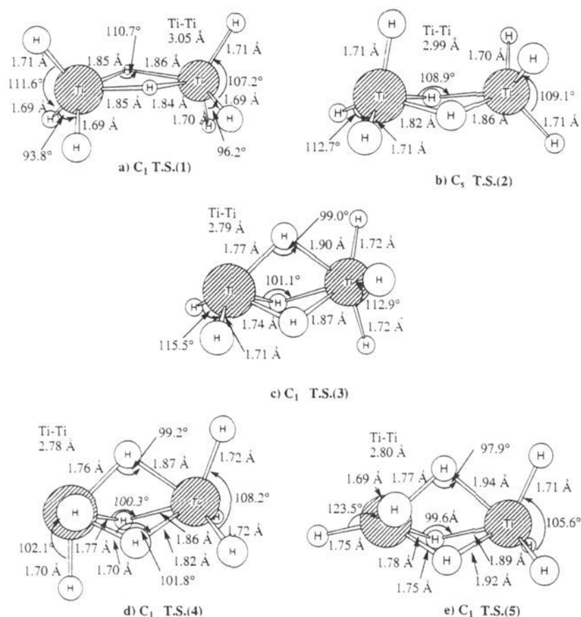
Figure 3. MP2/TZVP optimized structures which are transition states on the potential energy surface of \text{Ti}_2\text{H}_8 .
