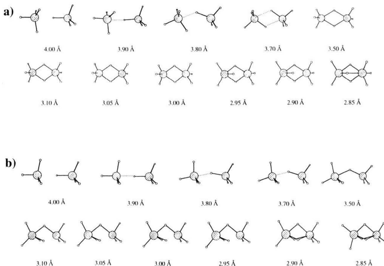
Figure 5. Each structure is the result of a constrained optimization at the RHF/TZVP level in which the Ti–Ti separation was “frozen” at the distance indicated: (a) represents a possible dimerization path to C_s(1) (Figure 2c), and (b) represents a possible dimerization path to C_s(4) (Figure 2f).
