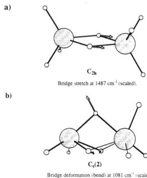
Figure 9. (a) Normal mode of the calculated frequency ( 1487\text{ cm}^{-1} scaled) that corresponds with a broad feature centered at 1490\text{ cm}^{-1} in the experimental spectrum. (b) Normal mode of the calculated frequency at 1081\text{ cm}^{-1} (scaled). This may correspond to the experimental peak found at 1140\text{ cm}^{-1} .
