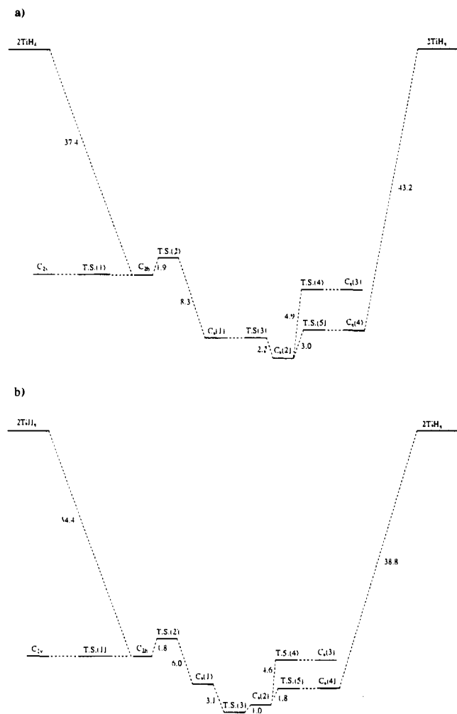
Figure 6. (a) CCSD(T)/TZVP(f) potential energy surface for \text{Ti}_2\text{H}_8 . (b) CCSD(T)/TZVP(f) potential energy surface for \text{Ti}_2\text{H}_8 with zero-point vibrational energy (calculated at the MP2/TZVP level) added. All energies are in \text{kcal mol}^{-1} (diagrams not to scale).
