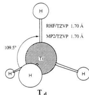
Figure 1. Titane equilibrium geometry.
