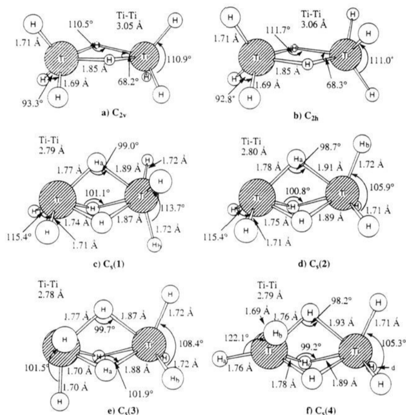
Figure 2. MP2/TZVP optimized structures which are minima on the potential energy surface of Ti 2 H 8 . In C s (1), C s (2), and C s (3) the two Ti's, H a , and H b are in the plane. In C s (4) The two Ti's, H a , H b , H c , and H d are in the plane.
