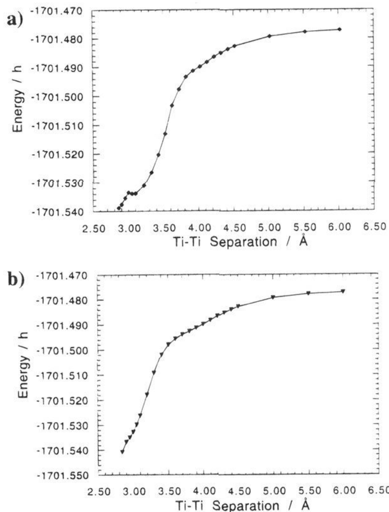
Figure 4. Plots of MP2/TZVP single-point energies in hartrees versus \text{Ti-Ti} separation in Å corresponding to (a) the dissociation of C_s(1) (Figure 2c) into two \text{TiH}_4 fragments and (b) the dissociation of C_s(4) (Figure 2f) into two \text{TiH}_4 fragments. The single-point energies were calculated at the constrained RHF/TZVP optimized geometries ( \text{Ti-Ti} distance constrained).
